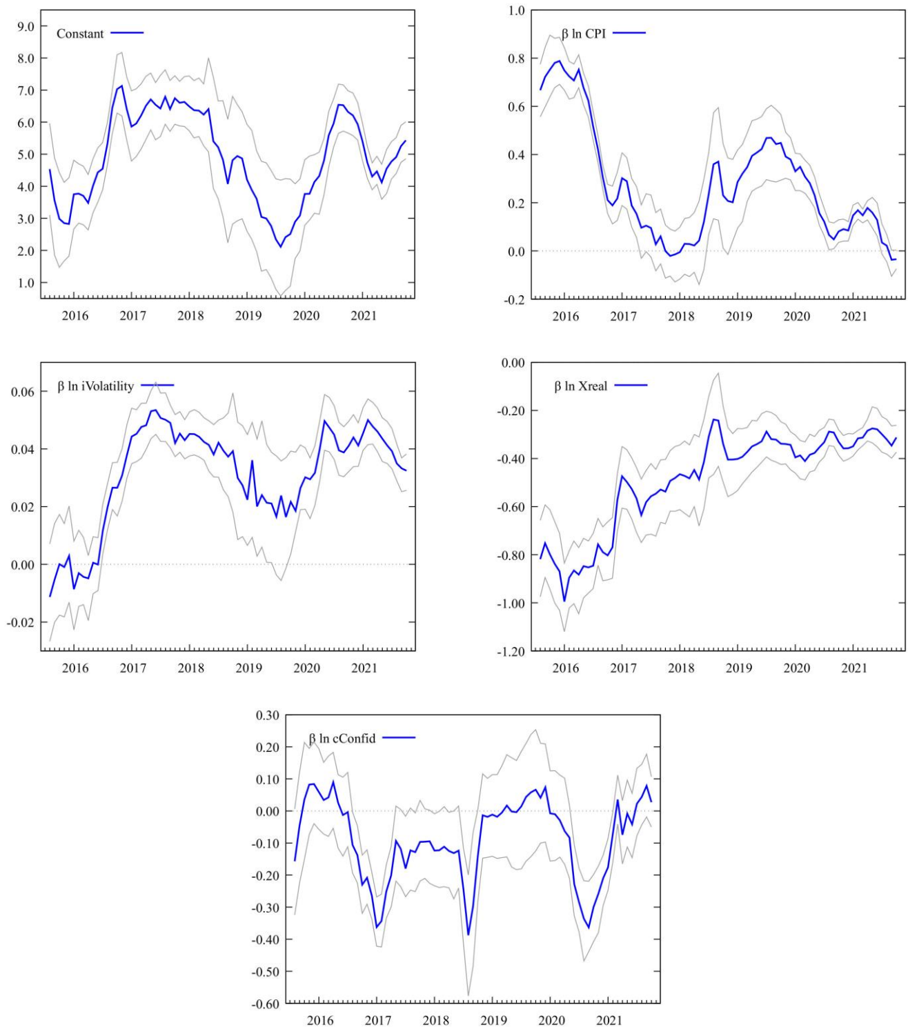
Figure 3: Rolling window coefficient estimates with 80% meboot confidence intervals.
